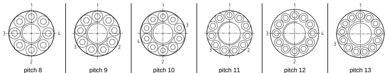
illustration 2: tightening of pressure screws
