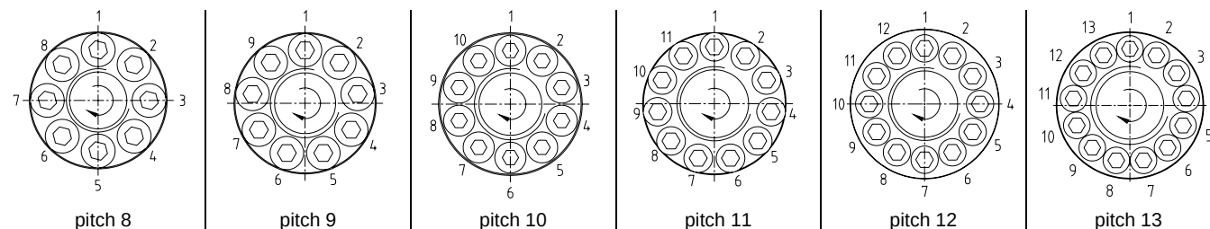
illustration 3: tightening of pressure screws (one after another)
